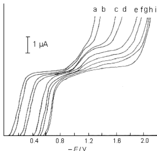
Figure 1 dc-Polarograms of 1 \times 10^{-4} mol L ^{-1} secnidazole in BR buffer solutions of different pH values: (a) 2.4; (b) 3.6; (c) 4.5; (d) 5.4; (e) 6.4; (f) 7.3; (g) 8.5; (h) 9.6; (i) 11.8.
