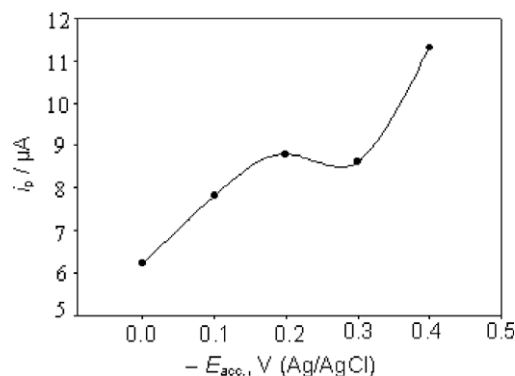
Figure 3 Effect of deposition potential on 5 \times 10^{-5} \text{ mol L}^{-1} secnidazole in BR buffer solution of pH 5.3 at t_{acc} = 60 \text{ s} , t = 500 \text{ mV s}^{-1} and step height = 5 \text{ mV} .
