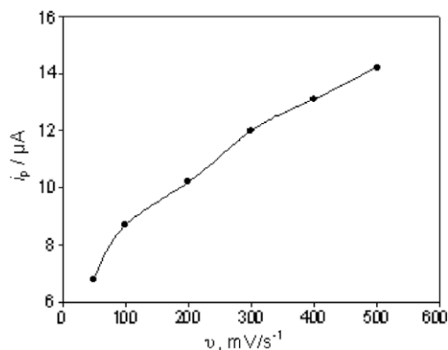
Figure 5 Effect of scan rate on 5 \times 10^{-5} \text{ mol L}^{-1} secnidazole in BR buffer solution of pH 5.3 at E_{\text{acc}} = -0.4 \text{ V} , t_{\text{acc}} = 30 \text{ s} and step height = 5 mV.
