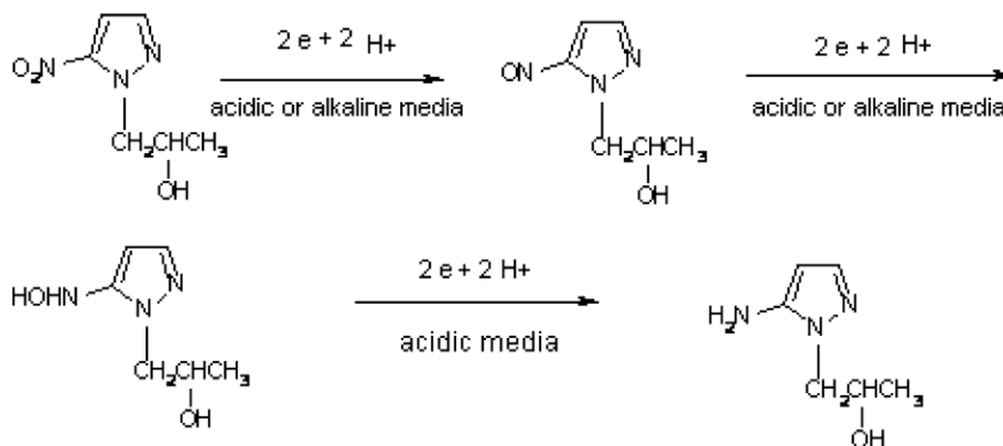
Scheme 2 Electrode reduction mechanism of secnidazole at different pH values.
