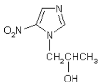
Scheme 1 Structural formula of secnidazole.
