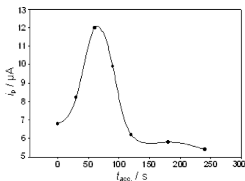
Figure 4 Effect of deposition time on 5 \times 10^{-5} \text{ mol L}^{-1} secnidazole in BR buffer solution of pH 5.3 at E_{\text{acc}} = -0.4 \text{ V} , t = 500 \text{ mV s}^{-1} and step height = 5 mV.
